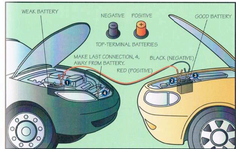
Correct jumper cable connections
