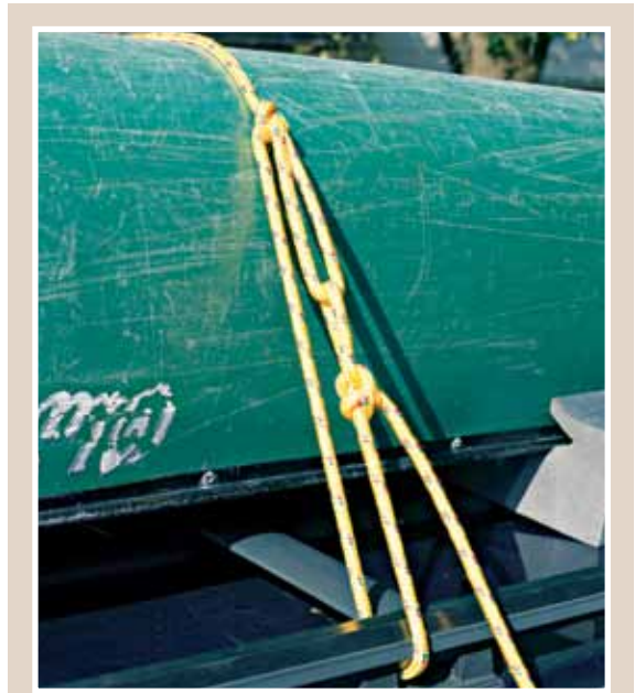
Ropes also work well to tie a boat to a rack. Instead of having a buckle or cam to secure the hull, use a bowline or a trucker's (or traveler's) hitch.
