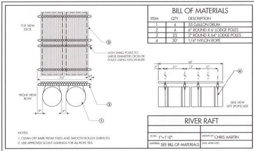
Orthographic projection: river raft
