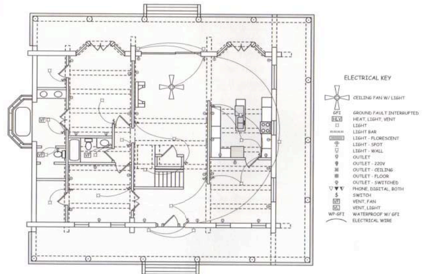
Electrical plan
