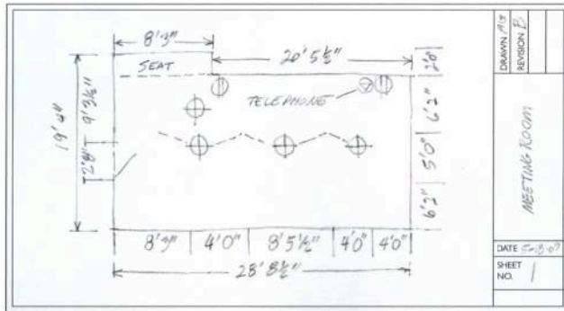
A freehand sketch
