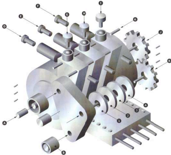
An exploded view shows the individual parts separated from one another but still in their correct relative positions.
