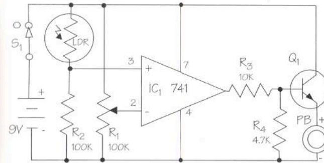
Electronics drawings include schematic diagrams (such as this one), block diagrams, logic diagrams, and wiring diagrams. Each has its own purpose and level of detail. For more about diagrams, see the Electronics and Radio merit badge pamphlets.
