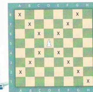
Figure 4. How the bishop moves
