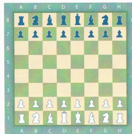
Figure 1. Starting positions for the chess pieces
