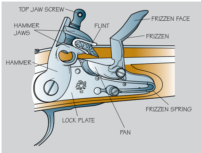
Flintlock action
