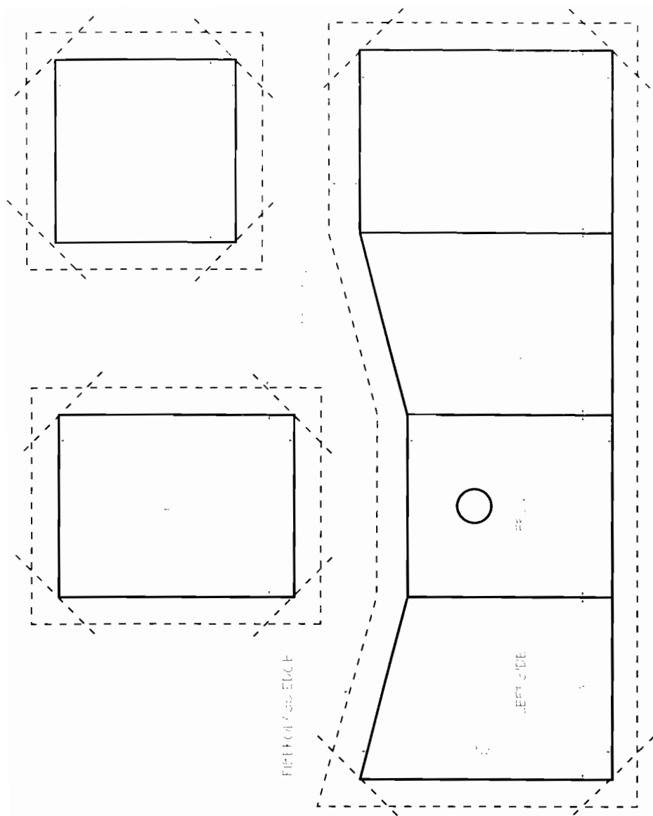
Template for cardboard walls, floor, and roof, to be enlarged. The fiberglass mat should be 1 inch wider than the cardboard.
