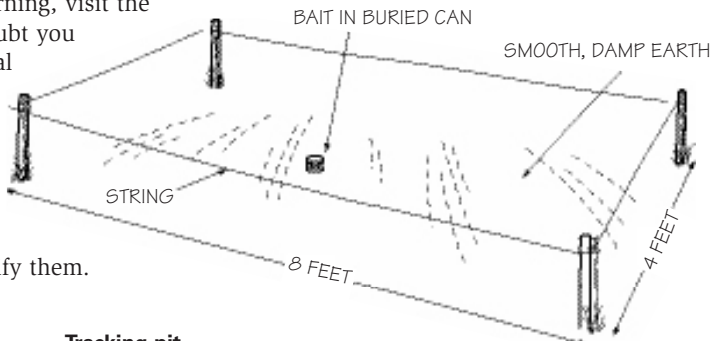
Tracking pit
